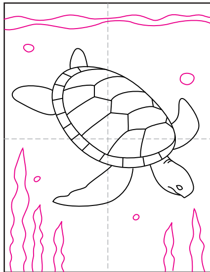
8. Add lots of seaweed and water line.
